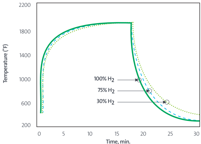
Figure 3: Effect of atmospheric composition on heating and cooling rates
