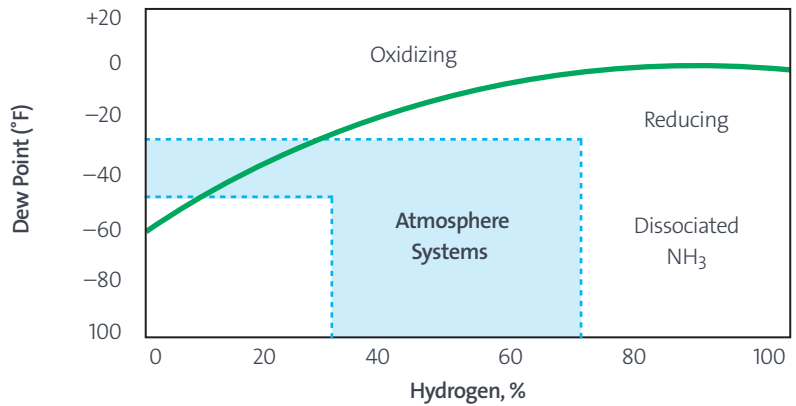
Figure 2: Oxidation reduction for 18% chromium stainless steel at 2000 °F
