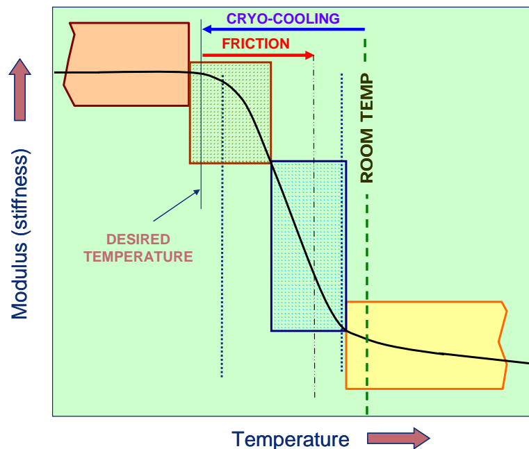
Figure 2: Typical stiffness curve for acrylic hydrophobic polymers showing need for cryogenic cooling during machining
